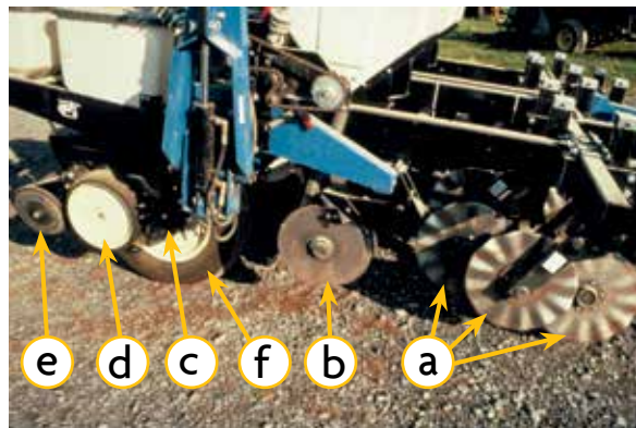
Figure 16.9. Zone-tilt planter: (a) coulters (cut up residues and break up soil in seed zone); (b) fertilizer disk openers (place granular starter fertilizer in a band next to the seed); (c) spider (trash) wheels (move residue away from the row); (d) seed placement unit; (e) press wheels (create firm seedbed); and (f) wheel used for transporting the planter.
